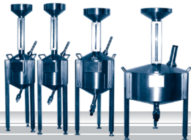
Eichkolben 2 x 10 Liter, 20 Liter, 50 Liter standard flasks 2 x10 litres, 20 litres, proving tanks 50 litres
